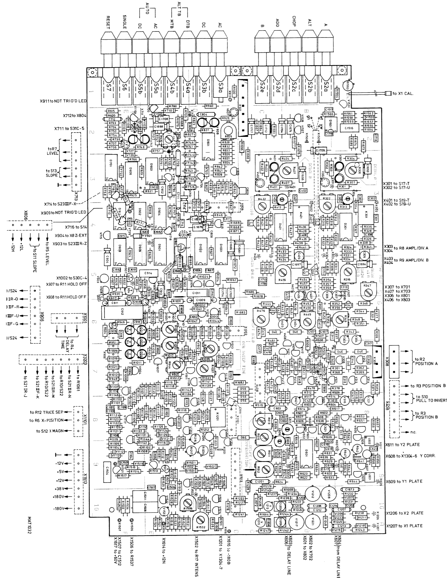
Component location amplifier unit.
